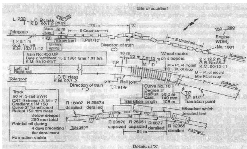
TYPICAL SKETCH OF ACCIDENT SITE
